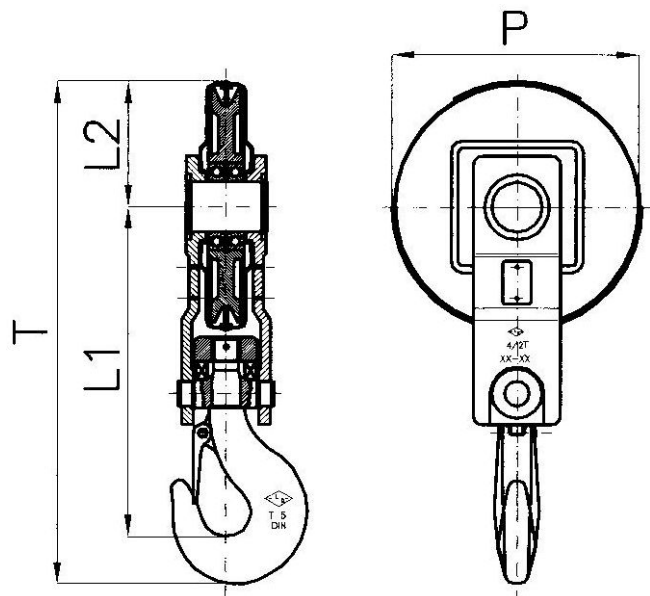
MOUFLE 1 REA CARTER ALUMINIUM
